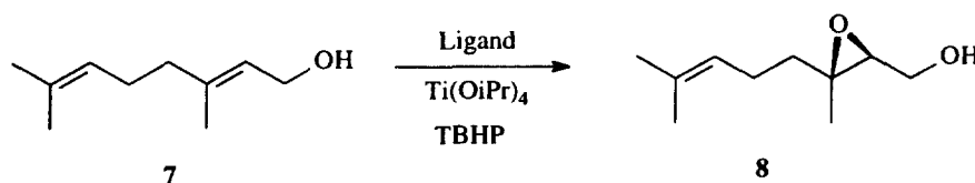
Scheme 3. Reagents and conditions: poly(tartrate ester), Ti(OPr i ) 4 , Bu t OOH (2 equiv.), 4 Å molecular sieves, CH 2 Cl 2
