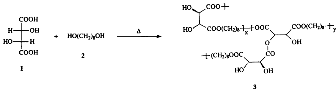
Scheme 1. Reagents and conditions: toluene p -sulfonic acid (3 mass%), 20 mol% excess of diol 2 , ca. 130°C, 4 days
